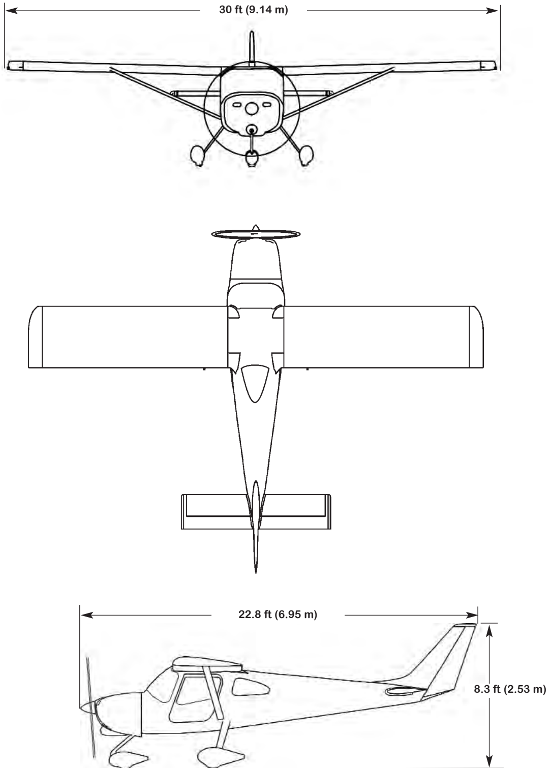
FIGURE I — MODEL 162 EXTERIOR DIMENSIONS
